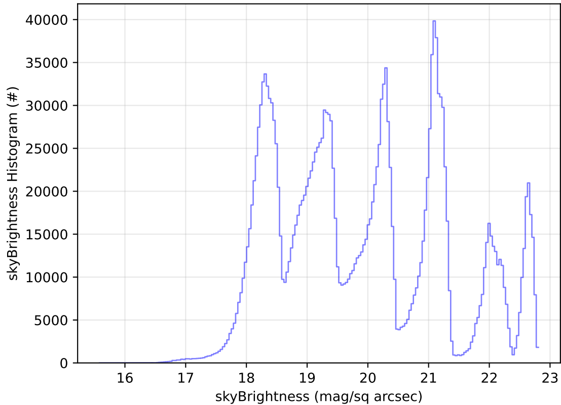
too_elab_2yr_r32_d2_ugrizy_v3.4_10yrs All sky all bands: skyBrightness Histogram
