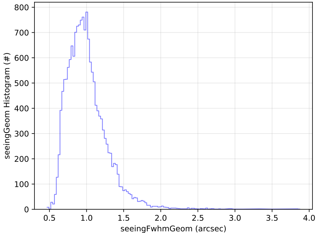
too_elab_2yr_r32_d2_ugrizy_v3.4_10yrs Yr 1 u band: seeingGeom Histogram
