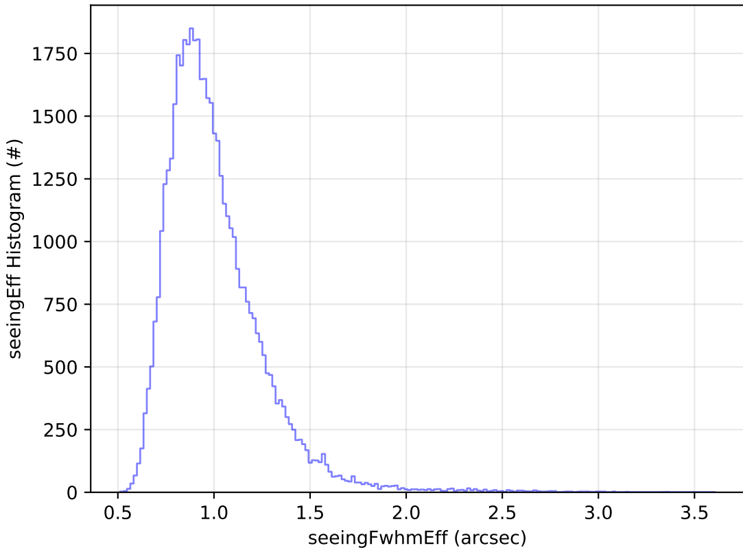
too_elab_2yr_r32_d2_ugrizy_v3.4_10yrs Yr 1 y band: seeingEff Histogram
