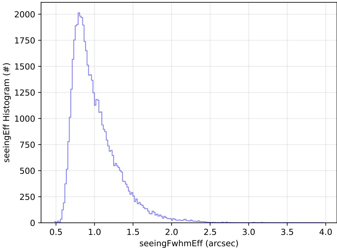
too_elab_2yr_r32_d2_ugrizy_v3.4_10yrs Yr 1 r band: seeingEff Histogram
