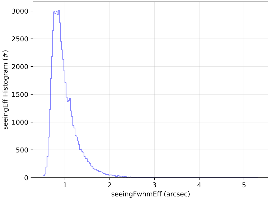
too_elab_2yr_r32_d2_ugrizy_v3.4_10yrs Yr 1 i band: seeingEff Histogram
