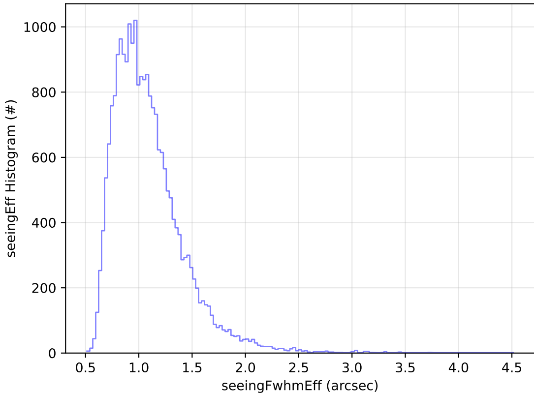
too_elab_2yr_r32_d2_ugrizy_v3.4_10yrs Yr 1 g band: seeingEff Histogram
