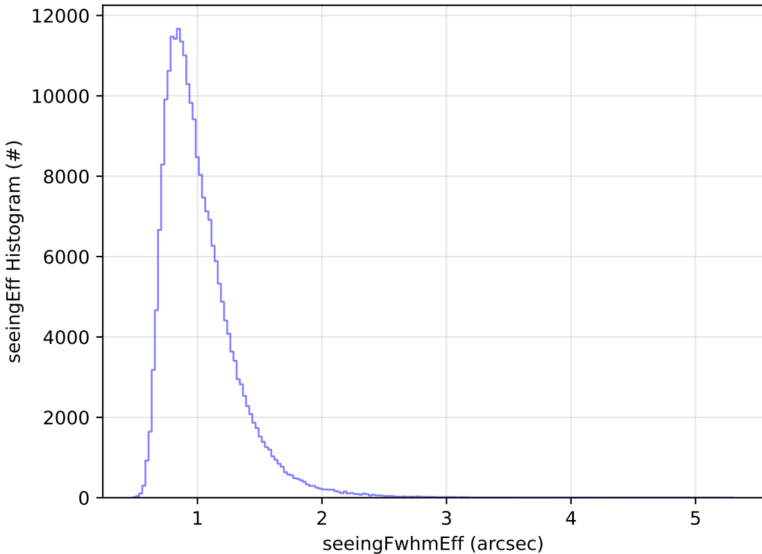
too_elab_2yr_r32_d2_ugrizy_v3.4_10yrs Yr 1 all bands: seeingEff Histogram
