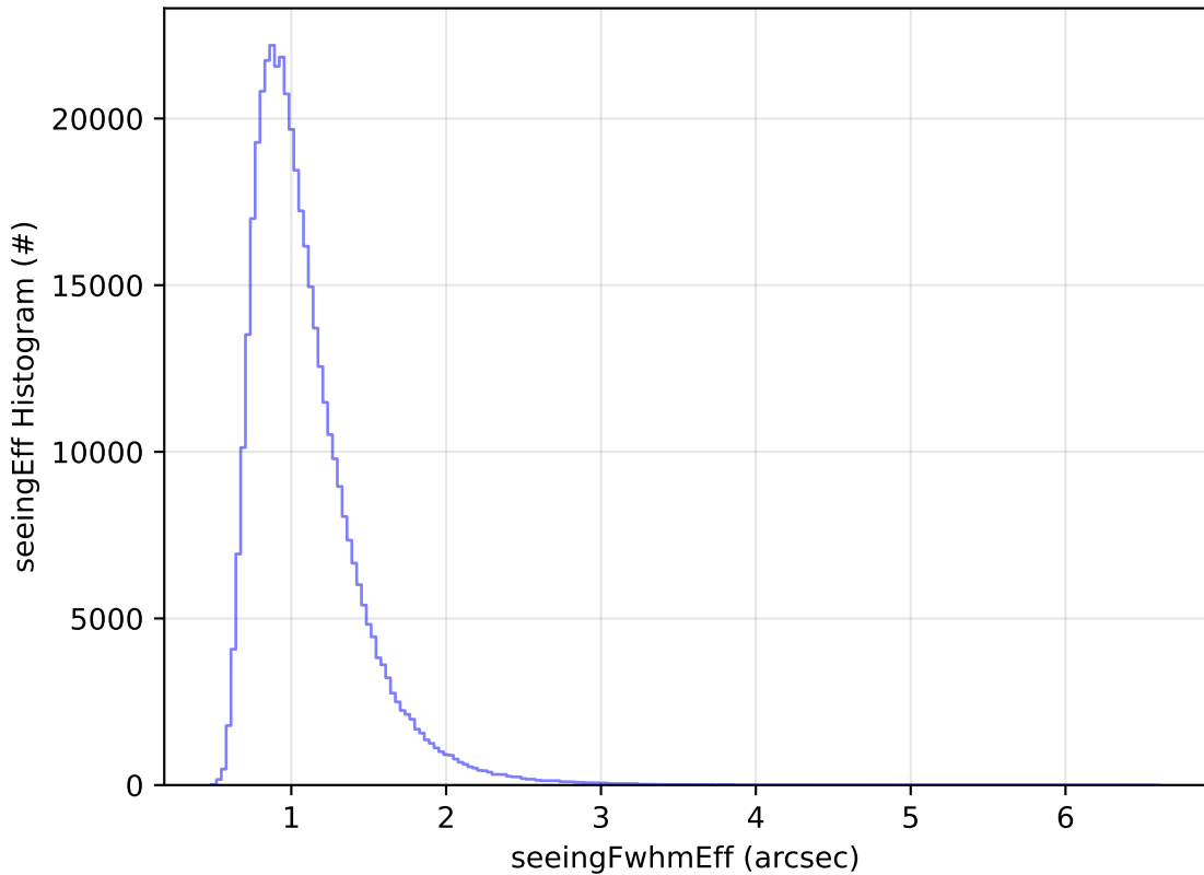
too_elab_2yr_r32_d2_ugrizy_v3.4_10yrs WFD z band: seeingEff Histogram
