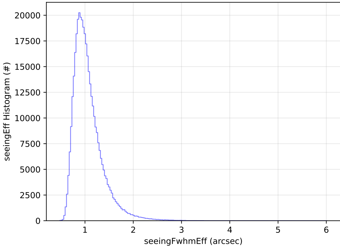
too_elab_2yr_r32_d2_ugrizy_v3.4_10yrs WFD y band: seeingEff Histogram
