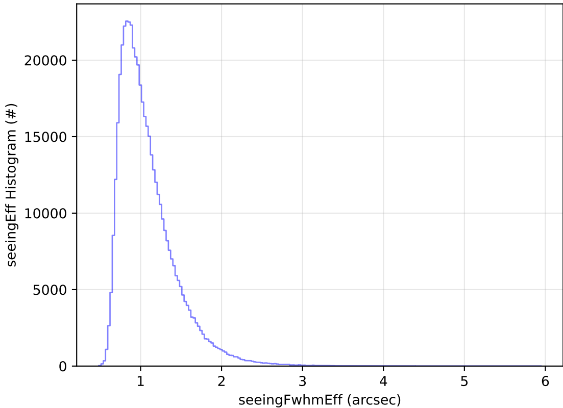
too_elab_2yr_r32_d2_ugrizy_v3.4_10yrs WFD i band: seeingEff Histogram
