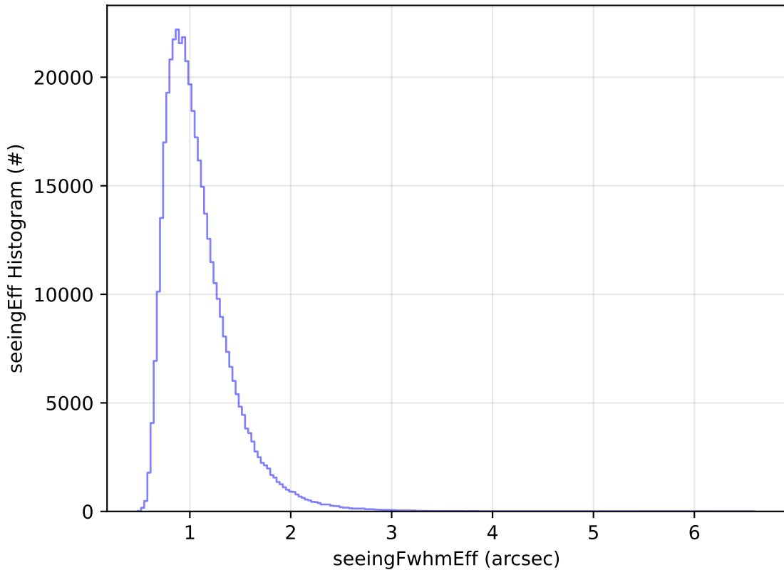
too_elab_2yr_r32_d2_ugrizy_v3.4_10yrs All sky z band: seeingEff Histogram
