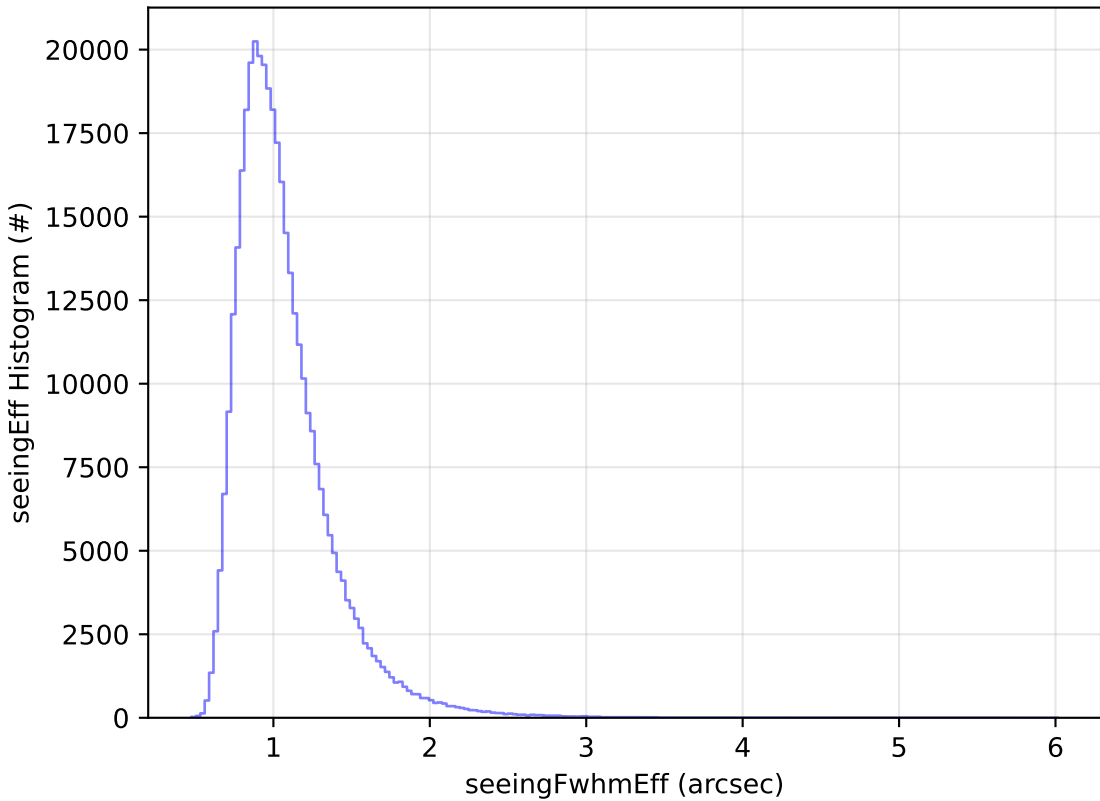
too_elab_2yr_r32_d2_ugrizy_v3.4_10yrs All sky y band: seeingEff Histogram
