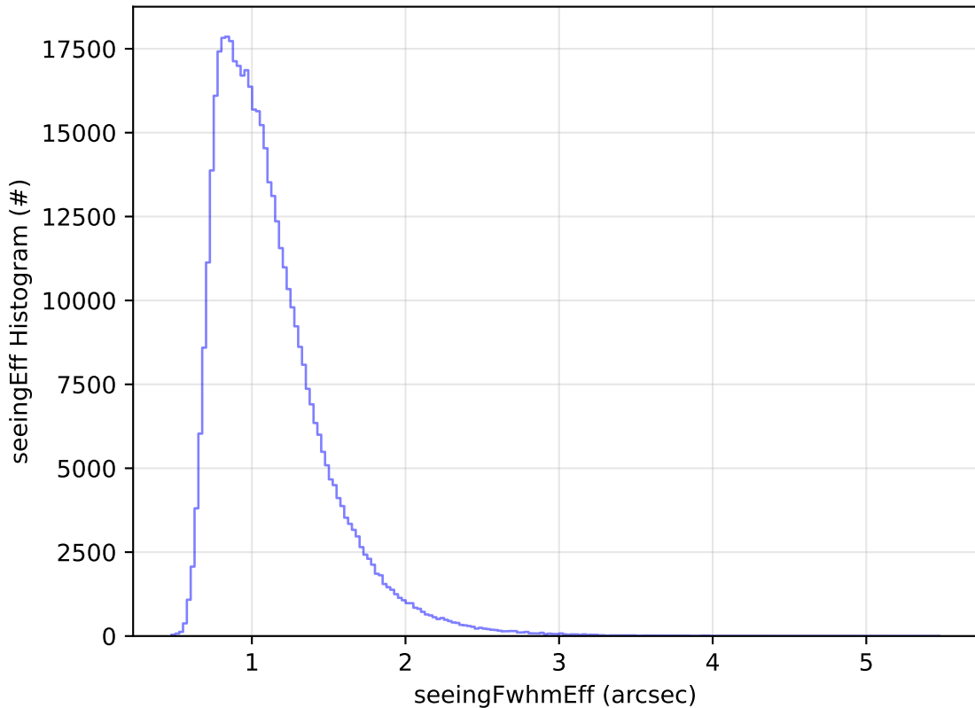
too_elab_2yr_r32_d2_ugrizy_v3.4_10yrs All sky r band: seeingEff Histogram
