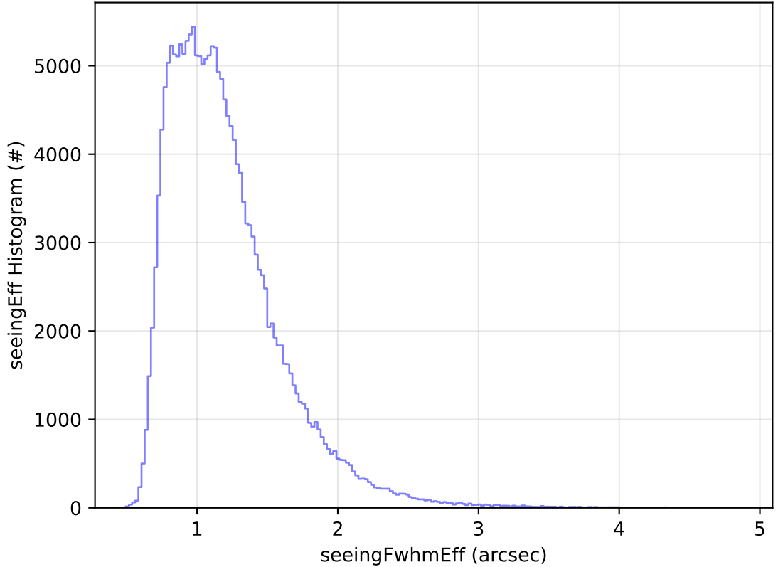
too_elab_2yr_r32_d2_ugrizy_v3.4_10yrs All sky g band: seeingEff Histogram
