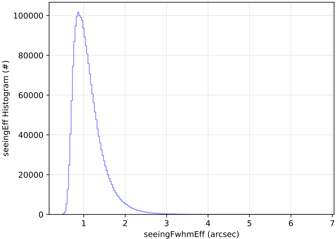
too_elab_2yr_r32_d2_ugrizy_v3.4_10yrs All sky all bands: seeingEff Histogram
