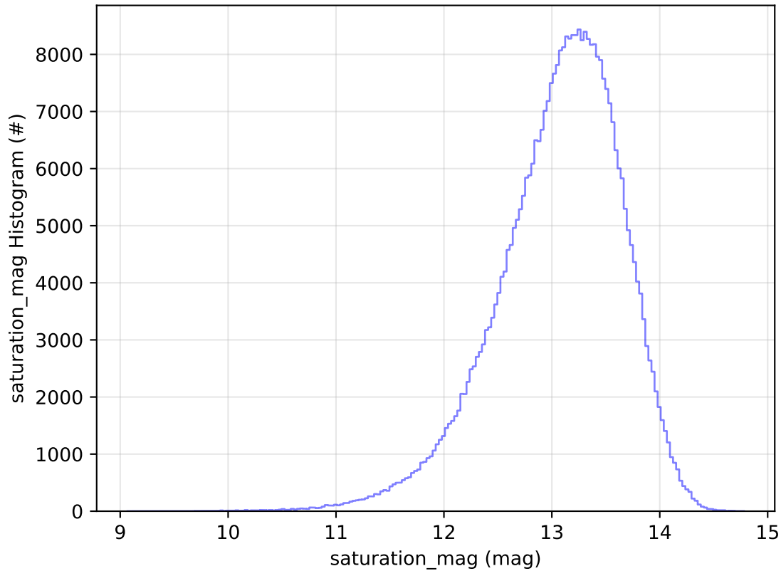
too_elab_2yr_r32_d2_ugrizy_v3.4_10yrs WFD y band: saturation_mag Histogram
