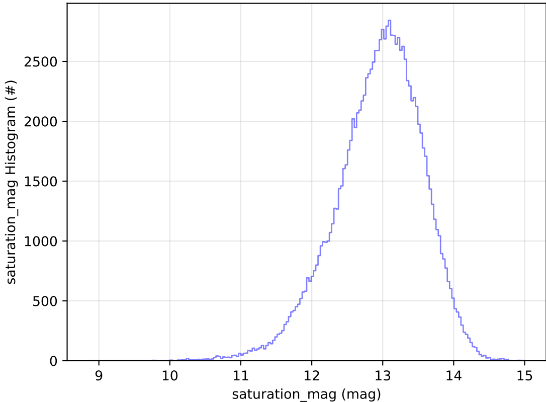
too_elab_2yr_r32_d2_ugrizy_v3.4_10yrs WFD u band: saturation_mag Histogram
