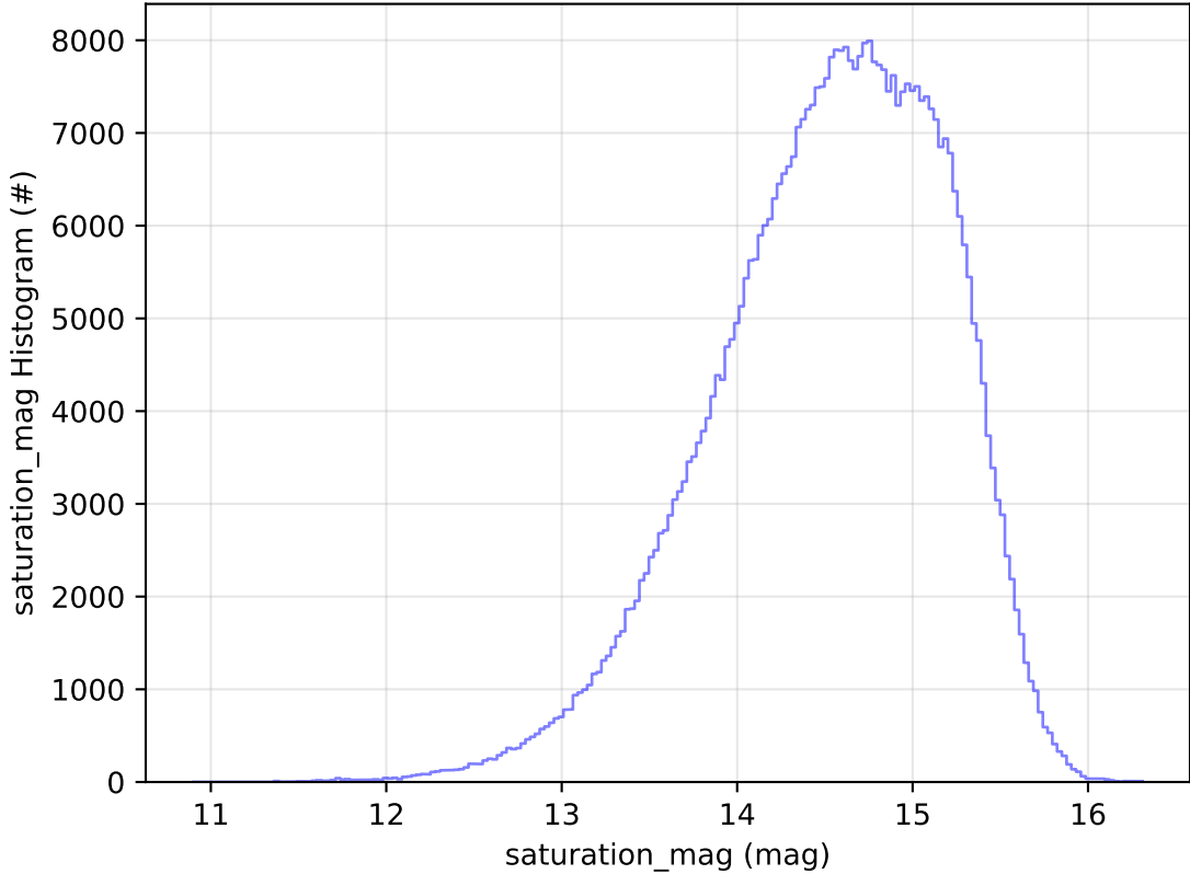
too_elab_2yr_r32_d2_ugrizy_v3.4_10yrs WFD r band: saturation_mag Histogram
