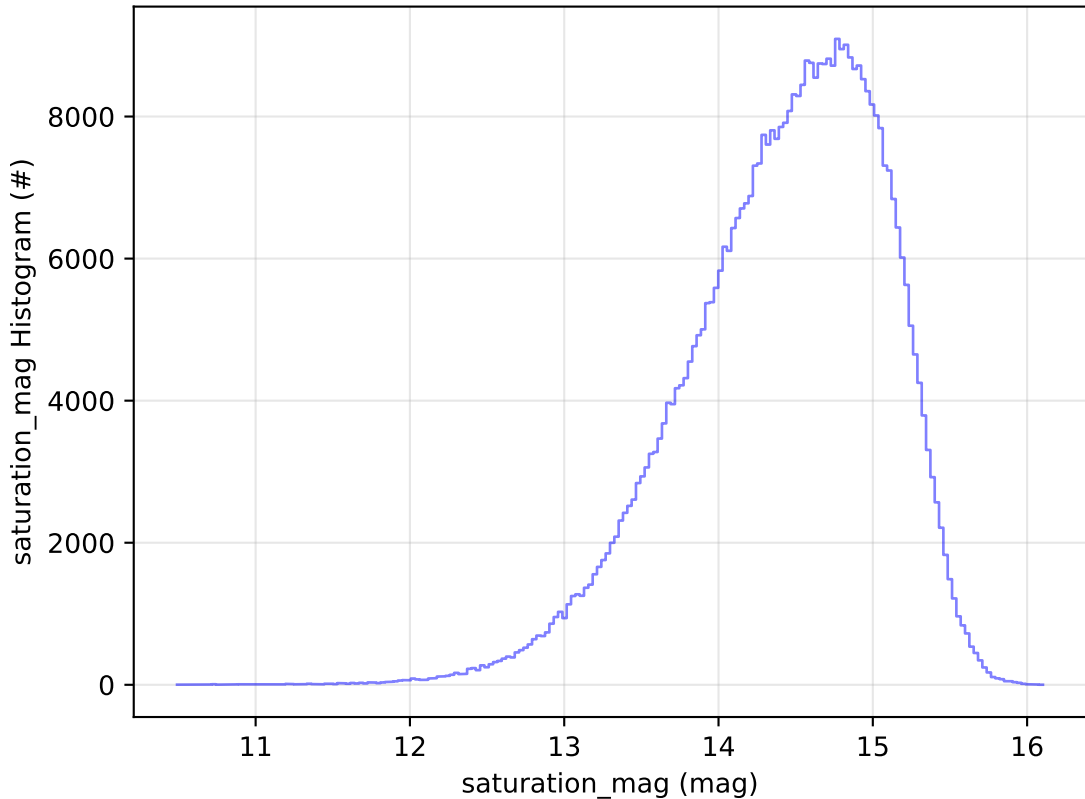
too_elab_2yr_r32_d2_ugrizy_v3.4_10yrs WFD i band: saturation_mag Histogram
