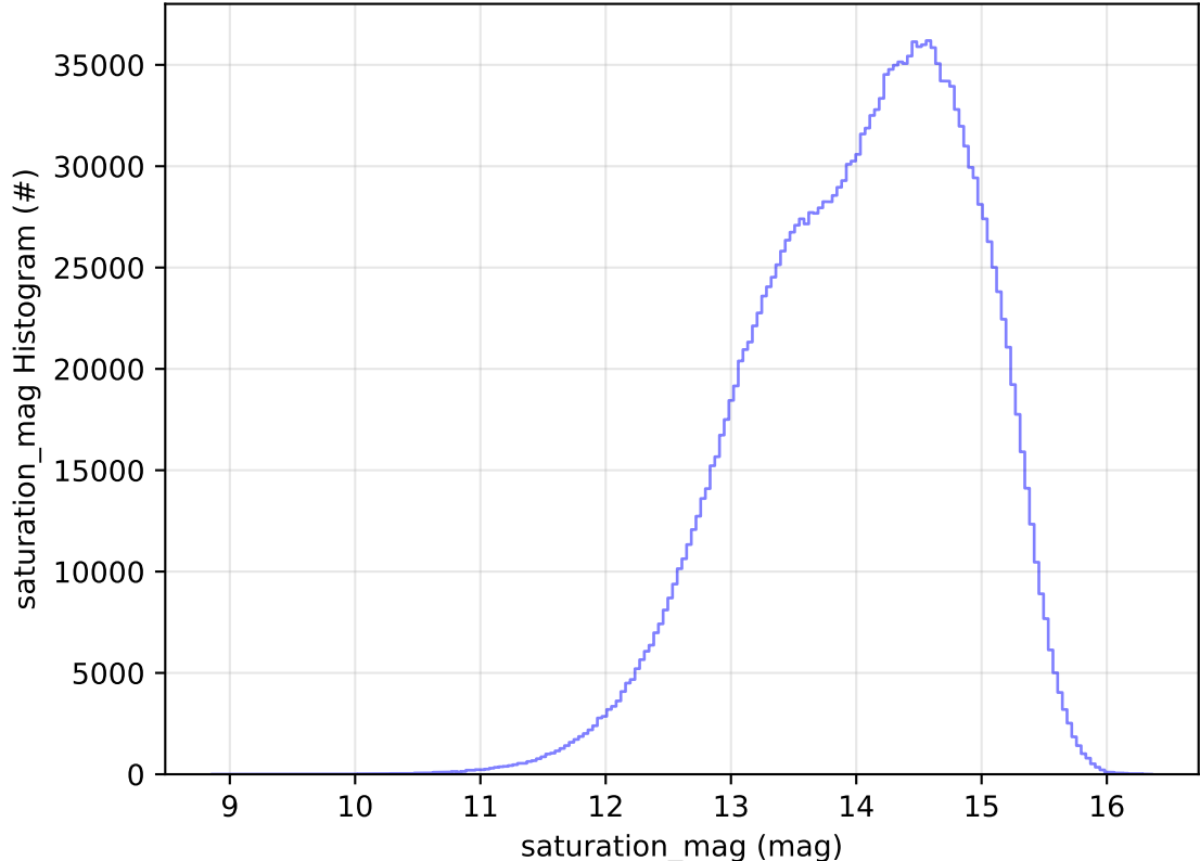
too_elab_2yr_r32_d2_ugrizy_v3.4_10yrs WFD all bands: saturation_mag Histogram
