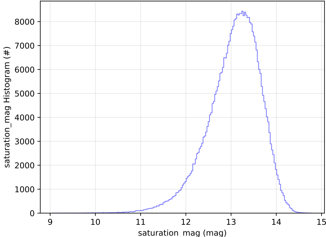
too_elab_2yr_r32_d2_ugrizy_v3.4_10yrs All sky y band: saturation_mag Histogram
