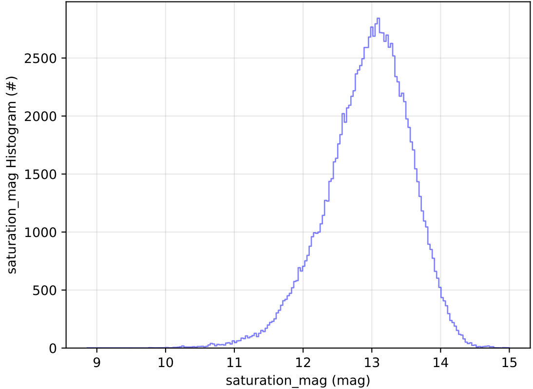
too_elab_2yr_r32_d2_ugrizy_v3.4_10yrs All sky u band: saturation_mag Histogram
