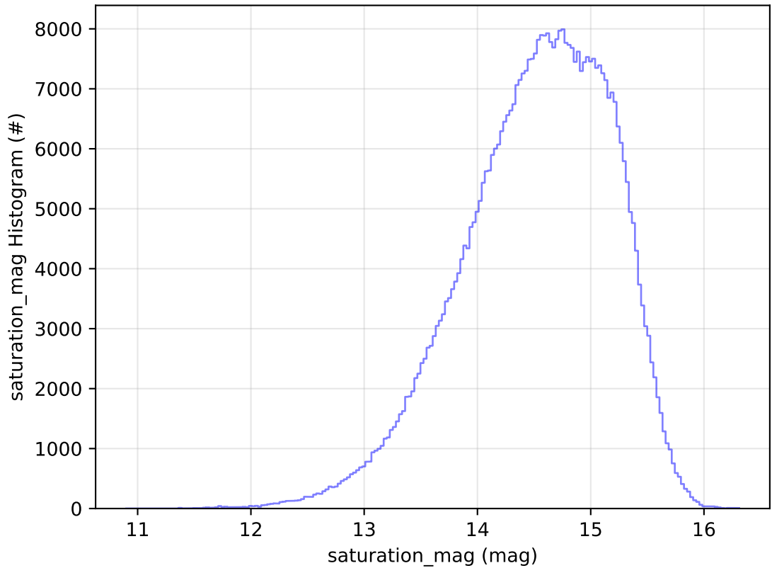
too_elab_2yr_r32_d2_ugrizy_v3.4_10yrs All sky r band: saturation_mag Histogram
