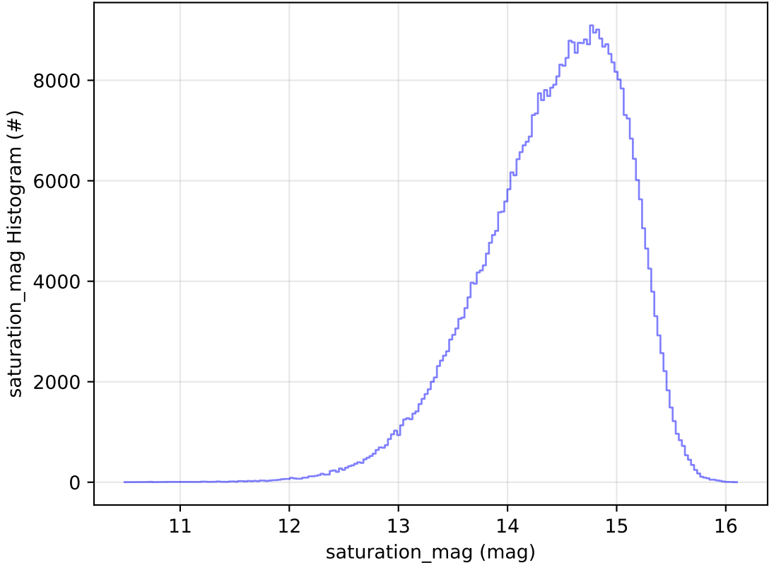
too_elab_2yr_r32_d2_ugrizy_v3.4_10yrs All sky i band: saturation_mag Histogram
