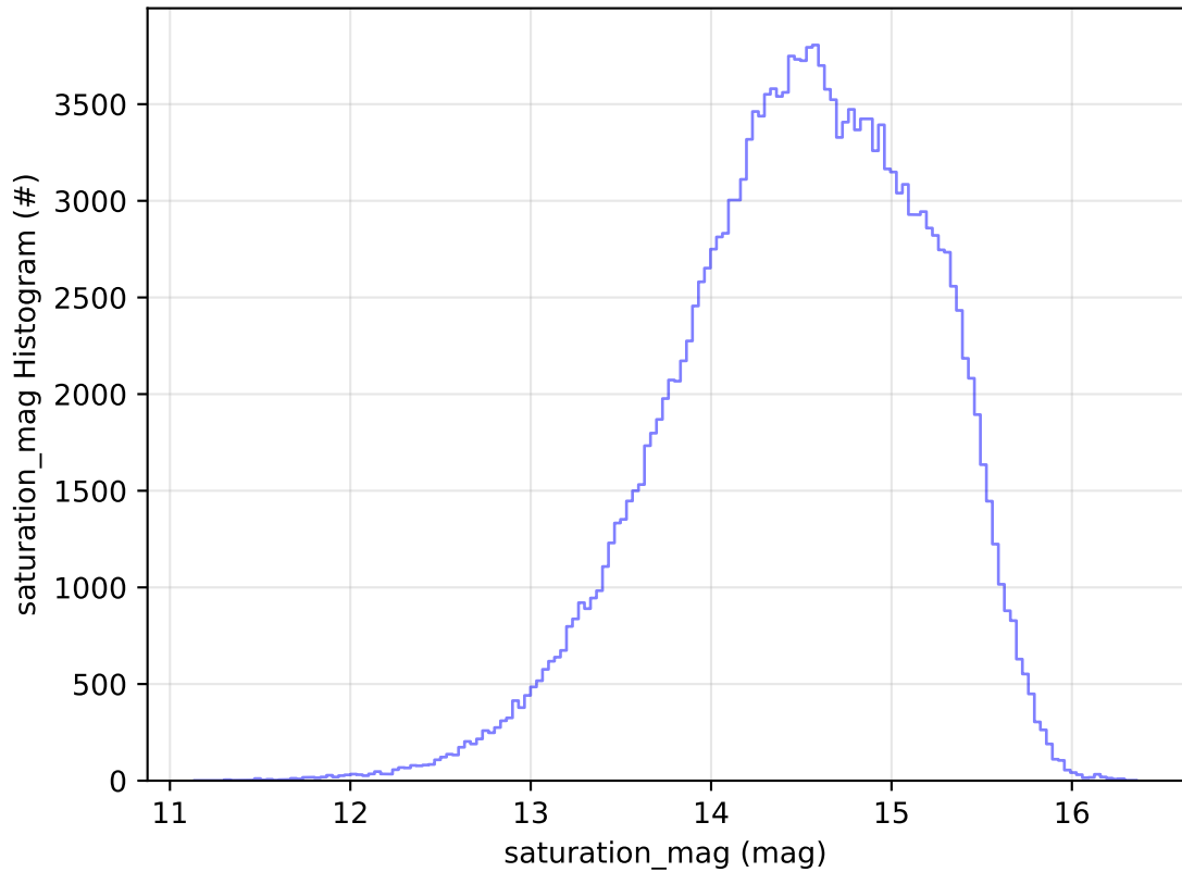
too_elab_2yr_r32_d2_ugrizy_v3.4_10yrs All sky g band: saturation_mag Histogram
