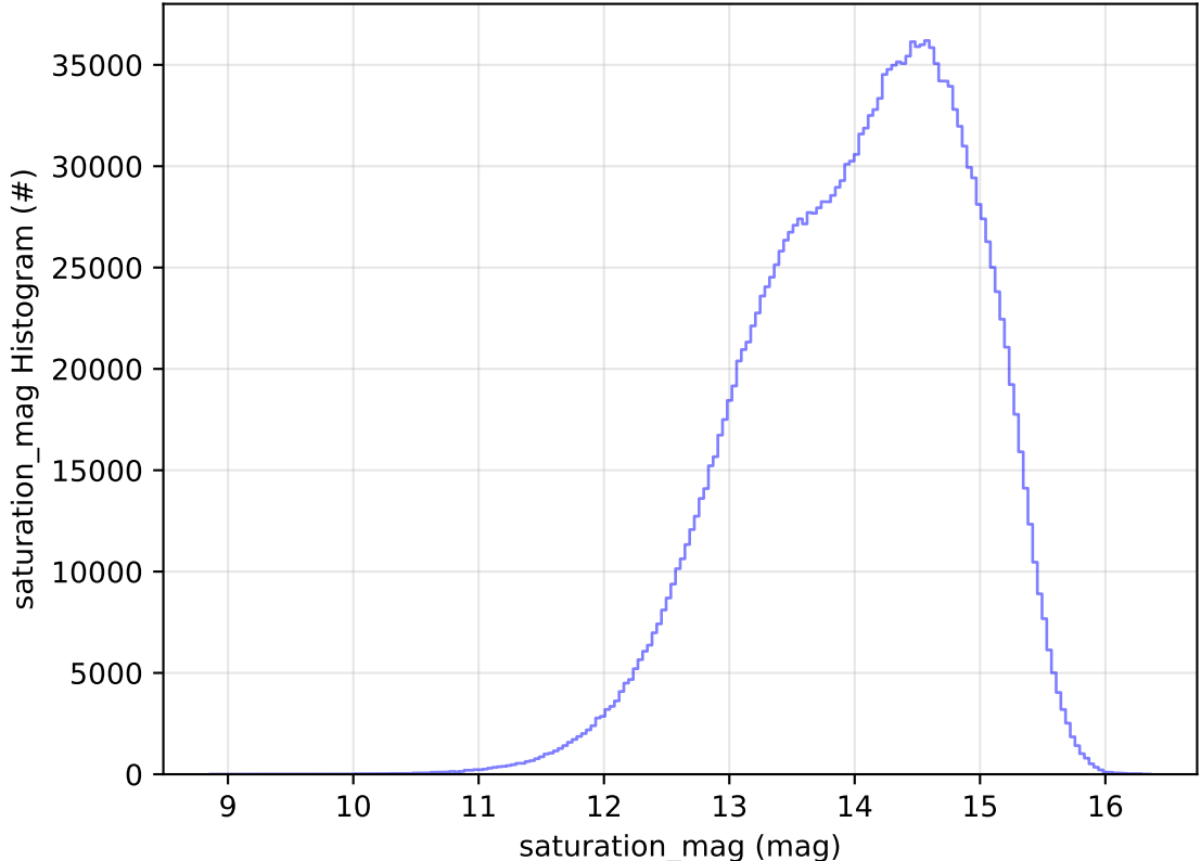
too_elab_2yr_r32_d2_ugrizy_v3.4_10yrs All sky all bands: saturation_mag Histogram
