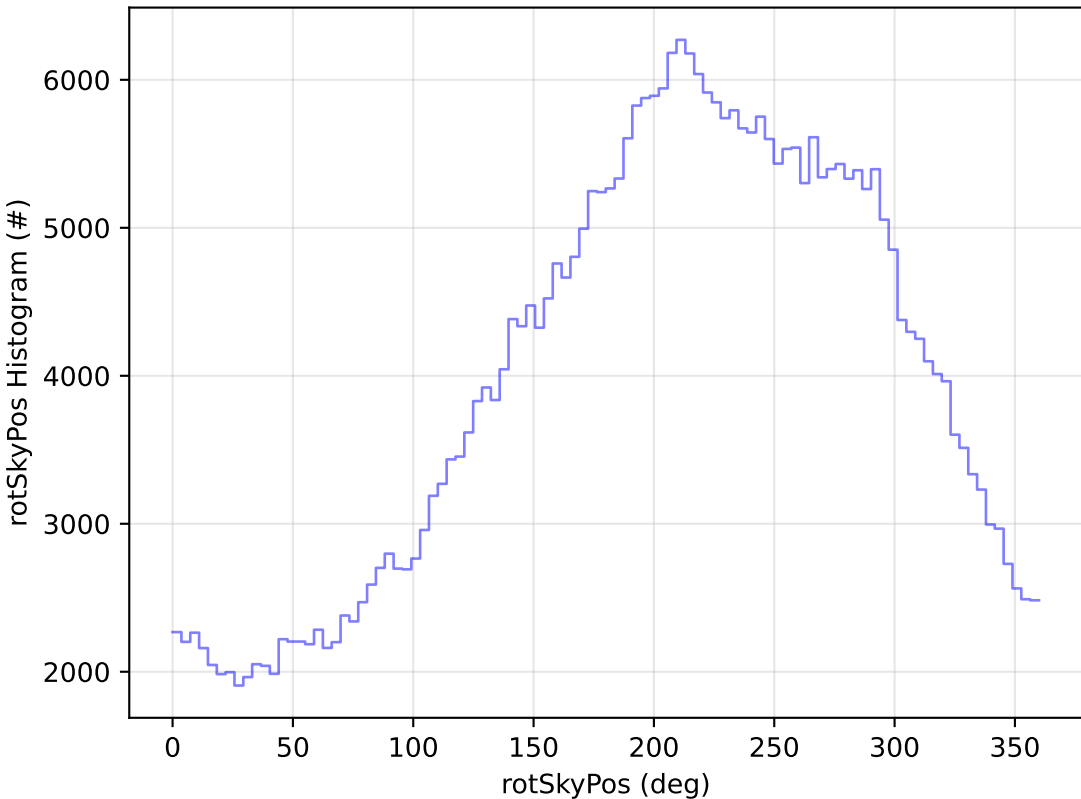
too_elab_2yr_r32_d2_ugrizy_v3.4_10yrs WFD y band: rotSkyPos Histogram
