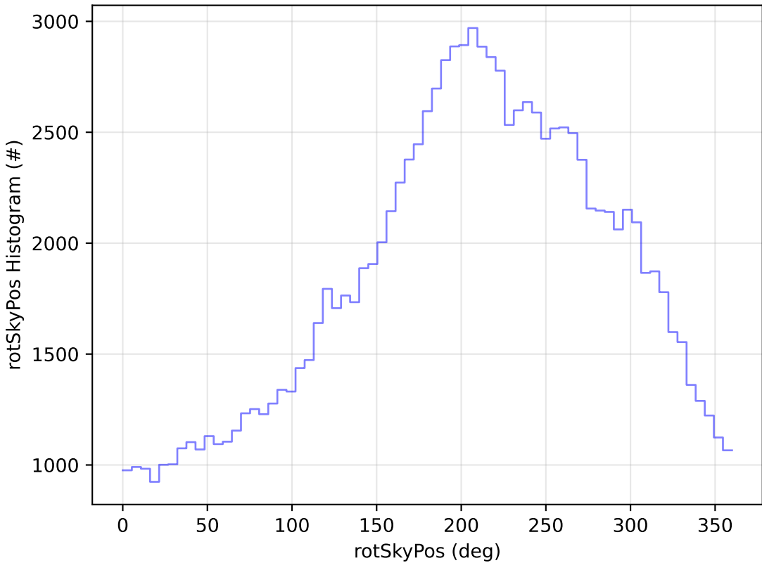
too_elab_2yr_r32_d2_ugrizy_v3.4_10yrs WFD u band: rotSkyPos Histogram
