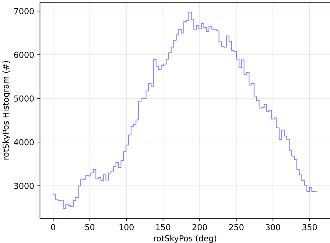
too_elab_2yr_r32_d2_ugrizy_v3.4_10yrs WFD r band: rotSkyPos Histogram
