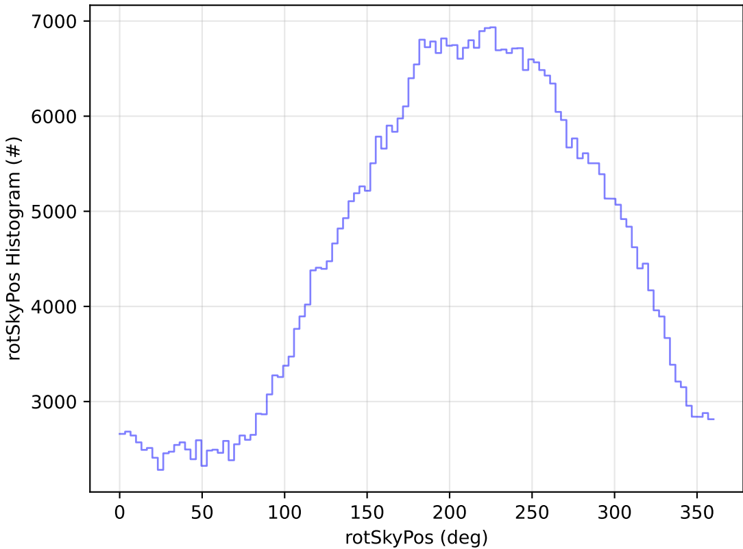
too_elab_2yr_r32_d2_ugrizy_v3.4_10yrs WFD i band: rotSkyPos Histogram
