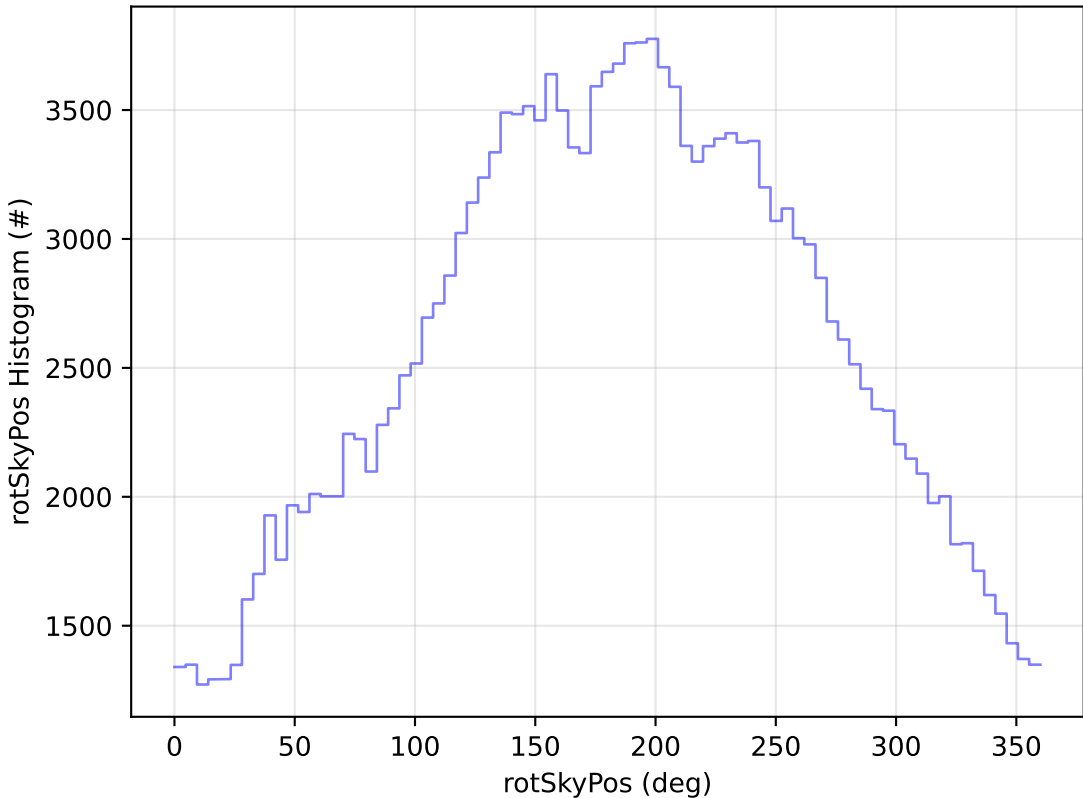
too_elab_2yr_r32_d2_ugrizy_v3.4_10yrs WFD g band: rotSkyPos Histogram
