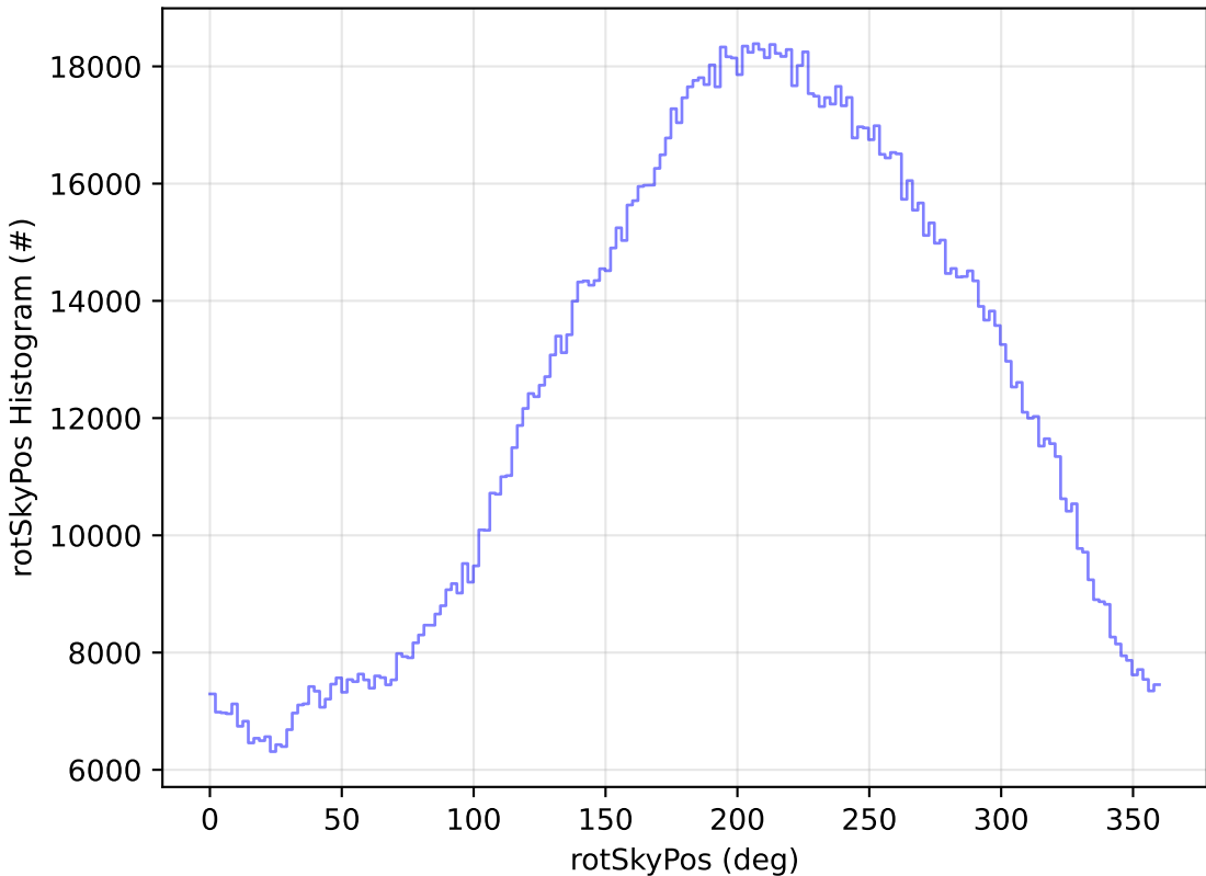
too_elab_2yr_r32_d2_ugrizy_v3.4_10yrs WFD all bands: rotSkyPos Histogram
