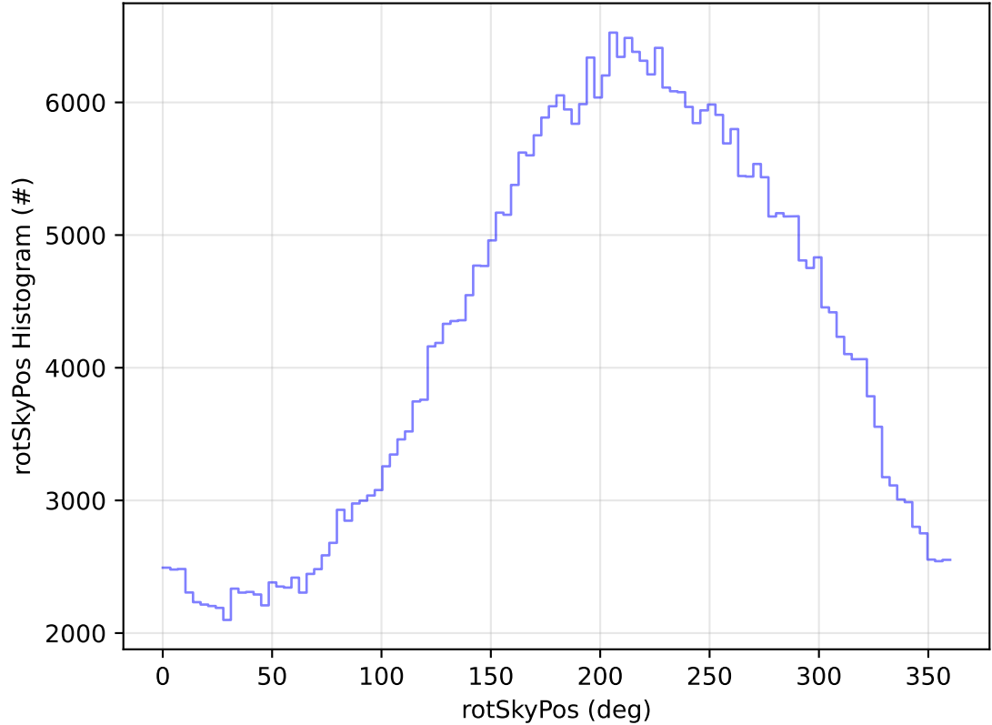
too_elab_2yr_r32_d2_ugrizy_v3.4_10yrs All sky z band: rotSkyPos Histogram
