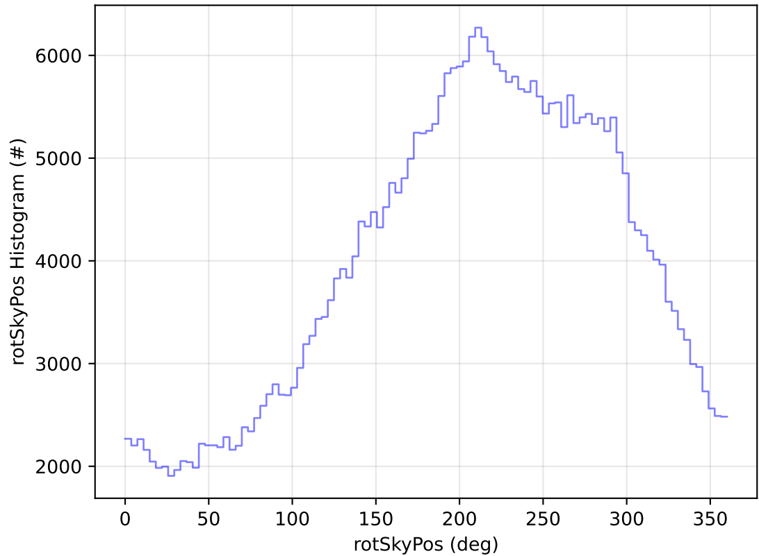
too_elab_2yr_r32_d2_ugrizy_v3.4_10yrs All sky y band: rotSkyPos Histogram
