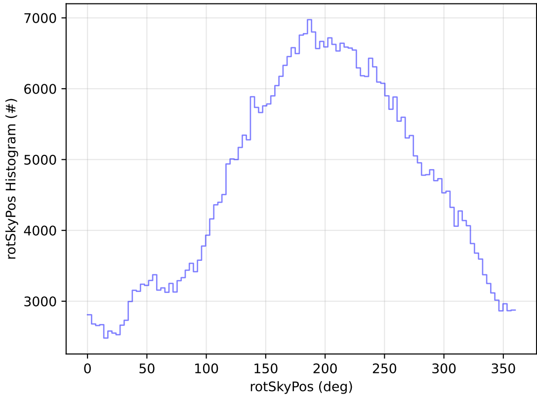
too_elab_2yr_r32_d2_ugrizy_v3.4_10yrs All sky r band: rotSkyPos Histogram
