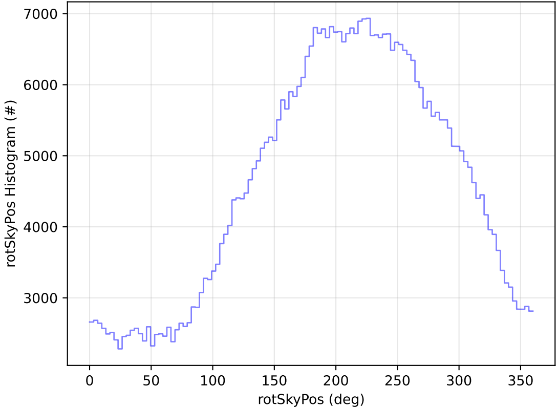
too_elab_2yr_r32_d2_ugrizy_v3.4_10yrs All sky i band: rotSkyPos Histogram
