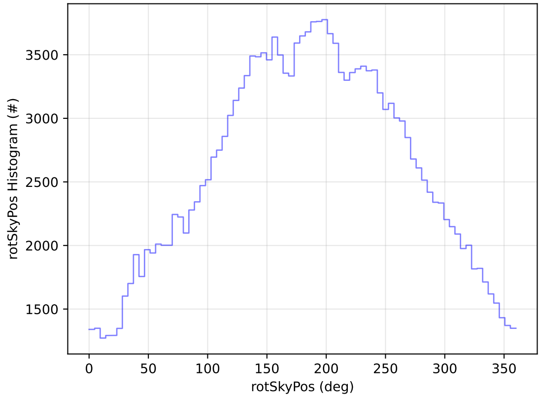
too_elab_2yr_r32_d2_ugrizy_v3.4_10yrs All sky g band: rotSkyPos Histogram
