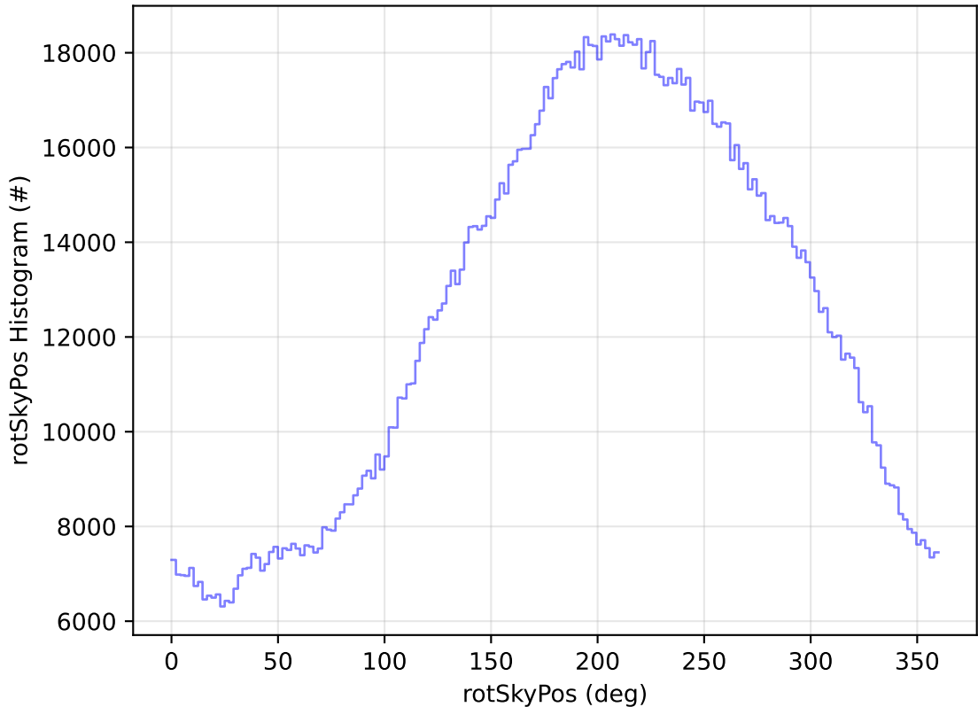
too_elab_2yr_r32_d2_ugrizy_v3.4_10yrs All sky all bands: rotSkyPos Histogram
