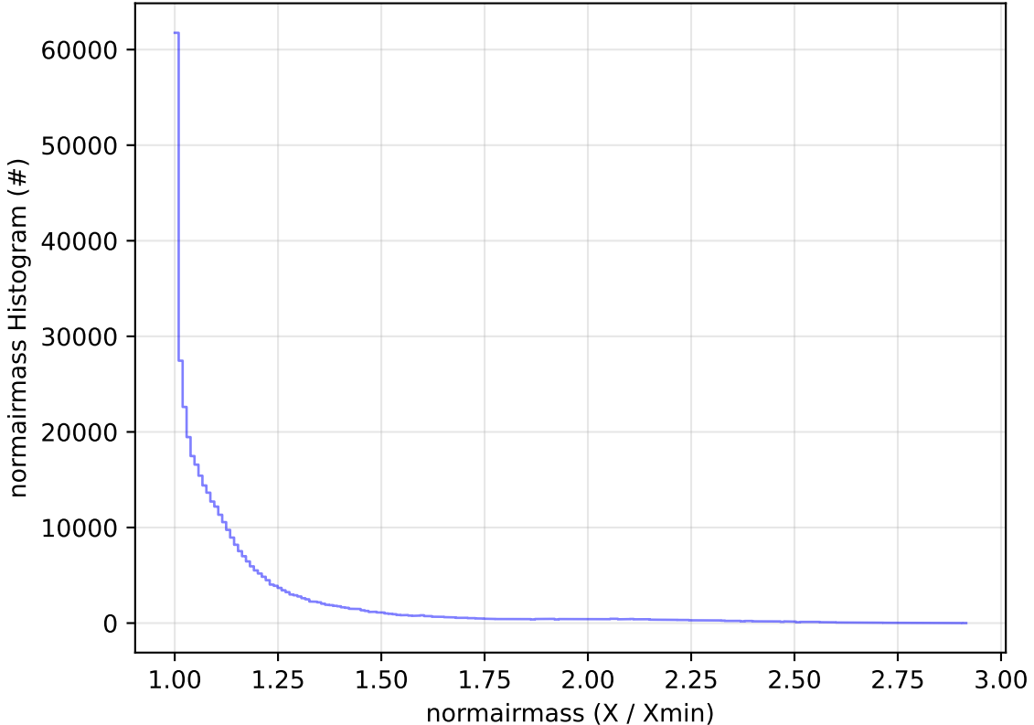
too_elab_2yr_r32_d2_ugrizy_v3.4_10yrs WFD z band: normairmass Histogram
