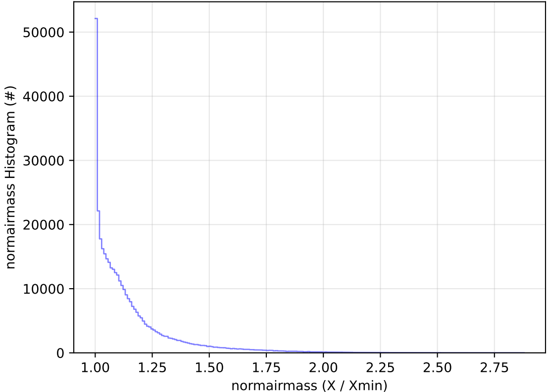
too_elab_2yr_r32_d2_ugrizy_v3.4_10yrs WFD y band: normairmass Histogram
