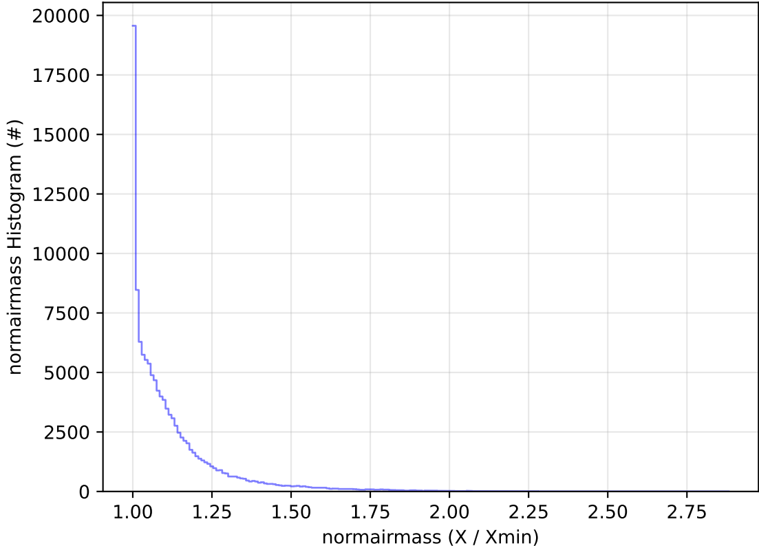
too_elab_2yr_r32_d2_ugrizy_v3.4_10yrs WFD u band: normairmass Histogram
