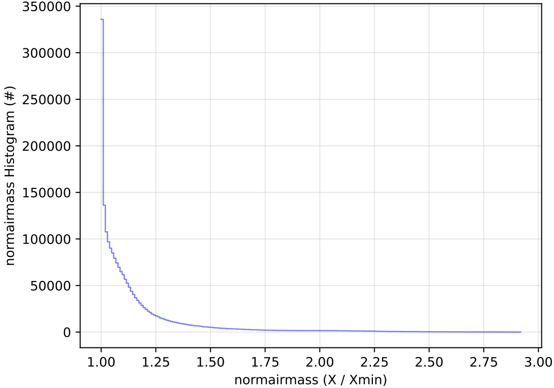
too_elab_2yr_r32_d2_ugrizy_v3.4_10yrs WFD all bands: normairmass Histogram
