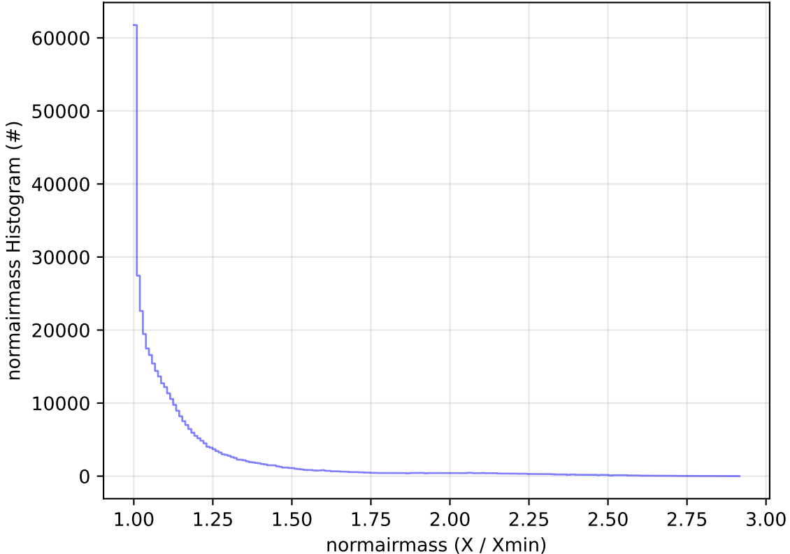
too_elab_2yr_r32_d2_ugrizy_v3.4_10yrs All sky z band: normairmass Histogram
