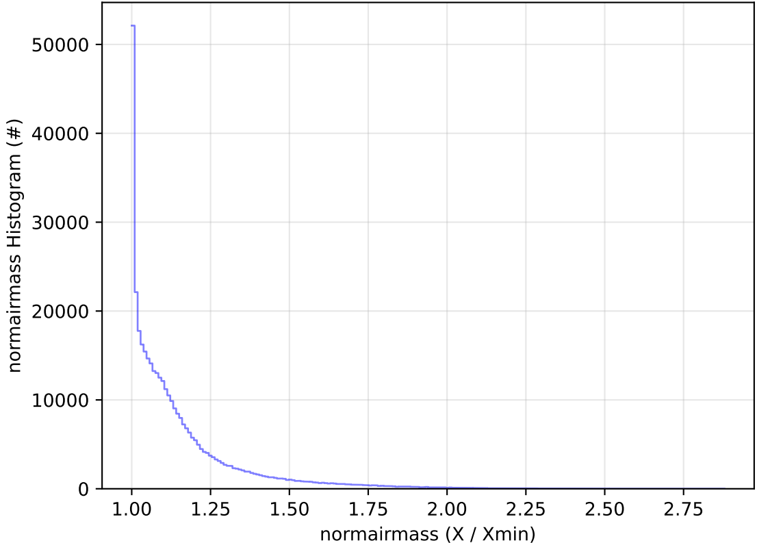
too_elab_2yr_r32_d2_ugrizy_v3.4_10yrs All sky y band: normairmass Histogram
