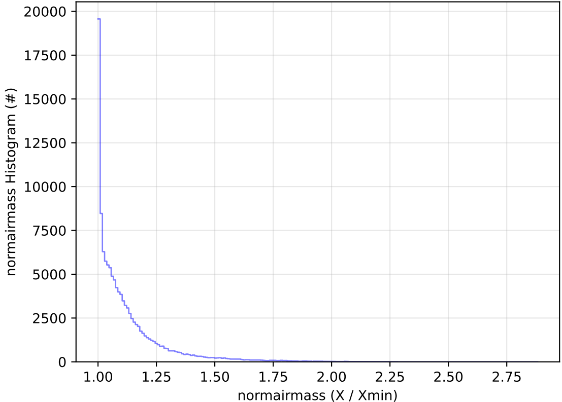
too_elab_2yr_r32_d2_ugrizy_v3.4_10yrs All sky u band: normairmass Histogram
