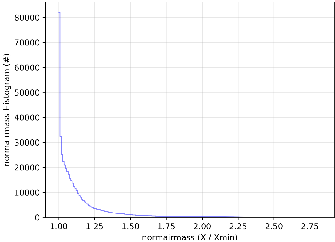
too_elab_2yr_r32_d2_ugrizy_v3.4_10yrs All sky r band: normairmass Histogram
