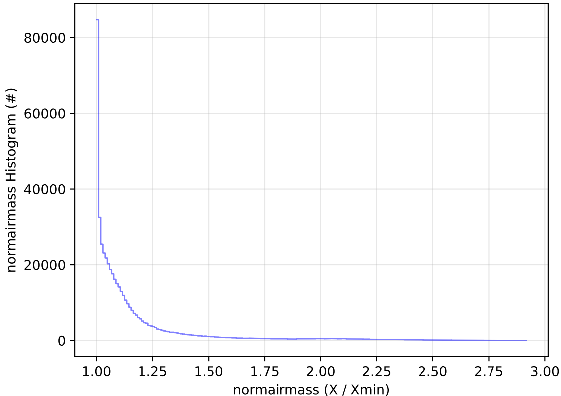
too_elab_2yr_r32_d2_ugrizy_v3.4_10yrs All sky i band: normairmass Histogram
