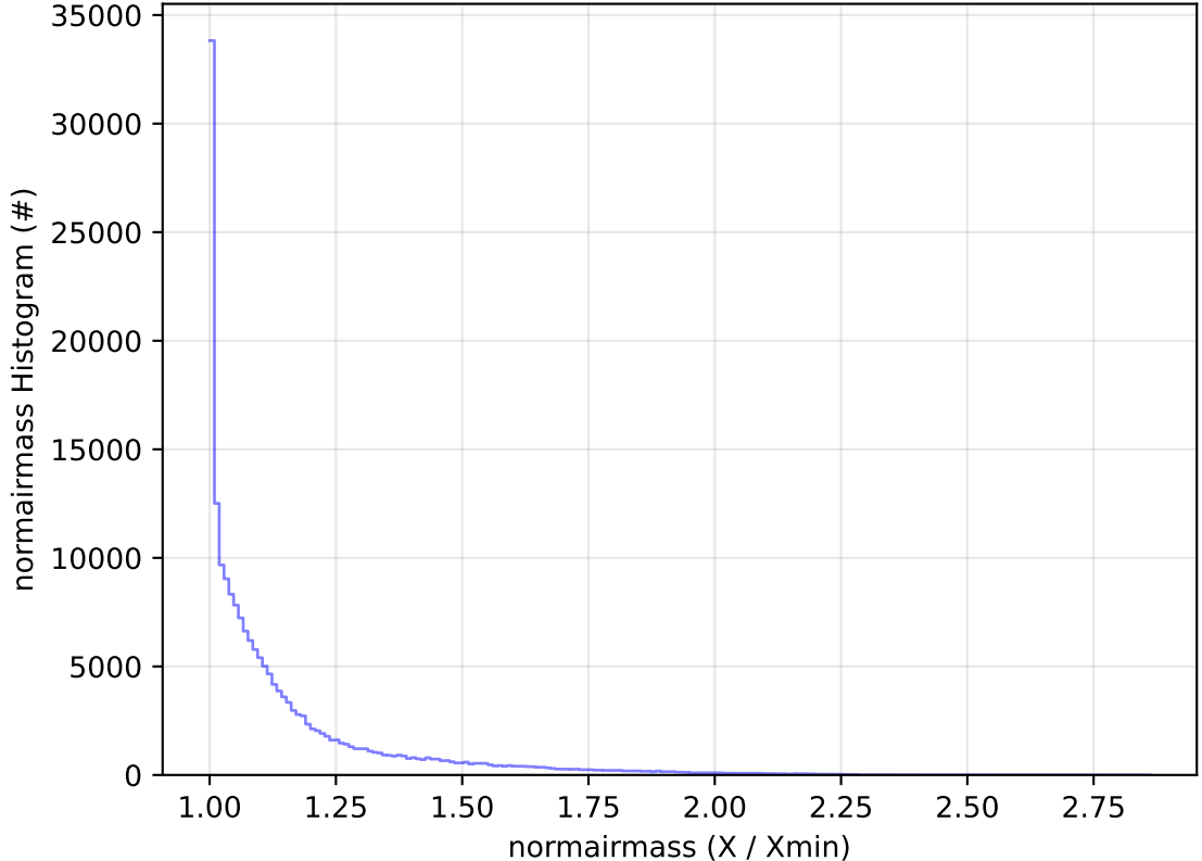
too_elab_2yr_r32_d2_ugrizy_v3.4_10yrs All sky g band: normairmass Histogram
