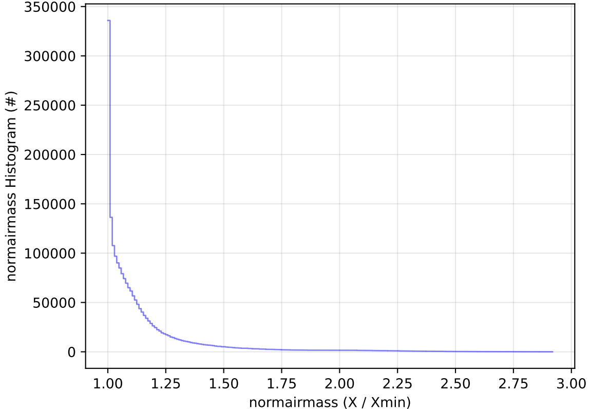
too_elab_2yr_r32_d2_ugrizy_v3.4_10yrs All sky all bands: normairmass Histogram
