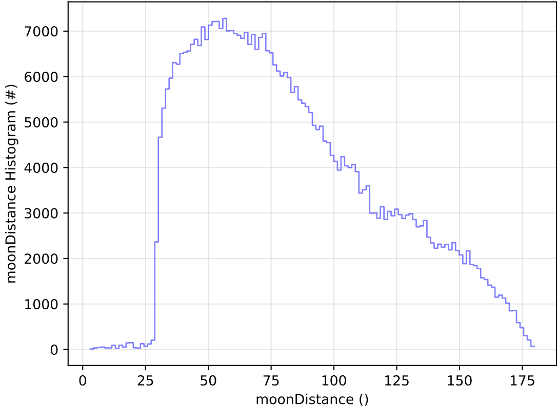
too_elab_2yr_r32_d2_ugrizy_v3.4_10yrs WFD z band: moonDistance Histogram
